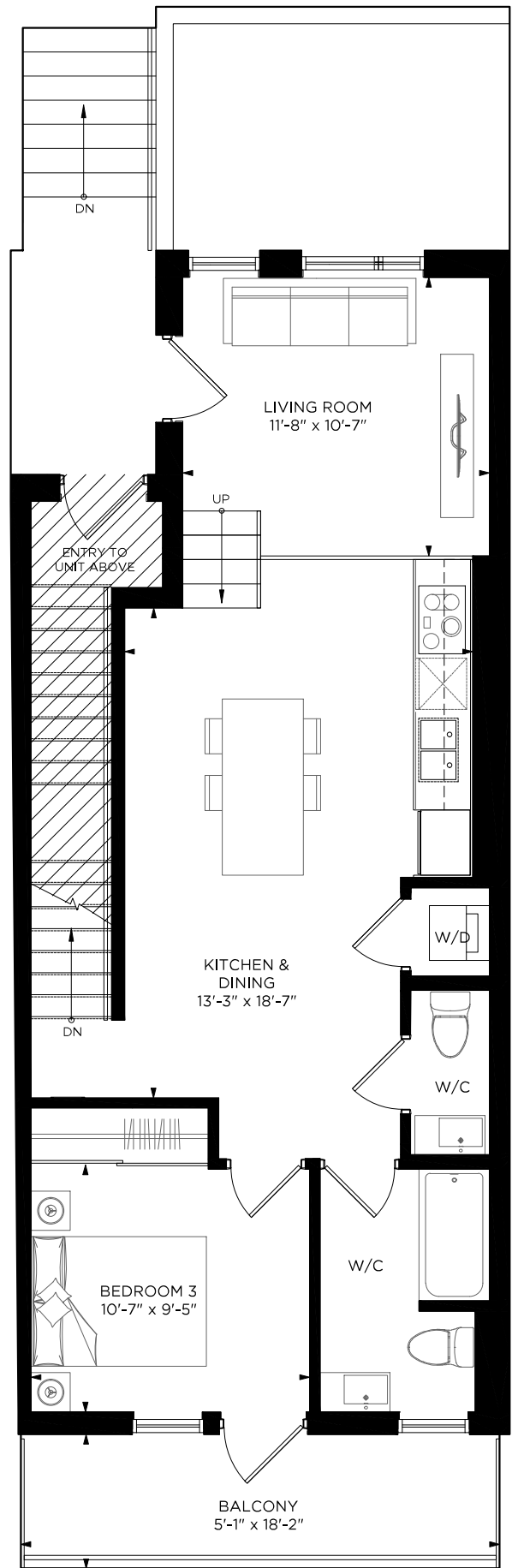
UPPER LEVEL GROUND FLOOR
