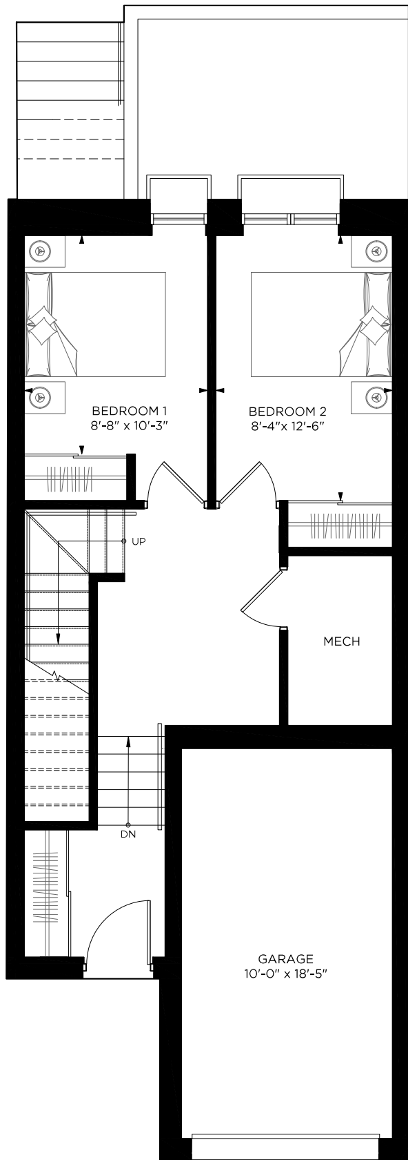
LOWER LEVEL BASEMENT FLOOR
