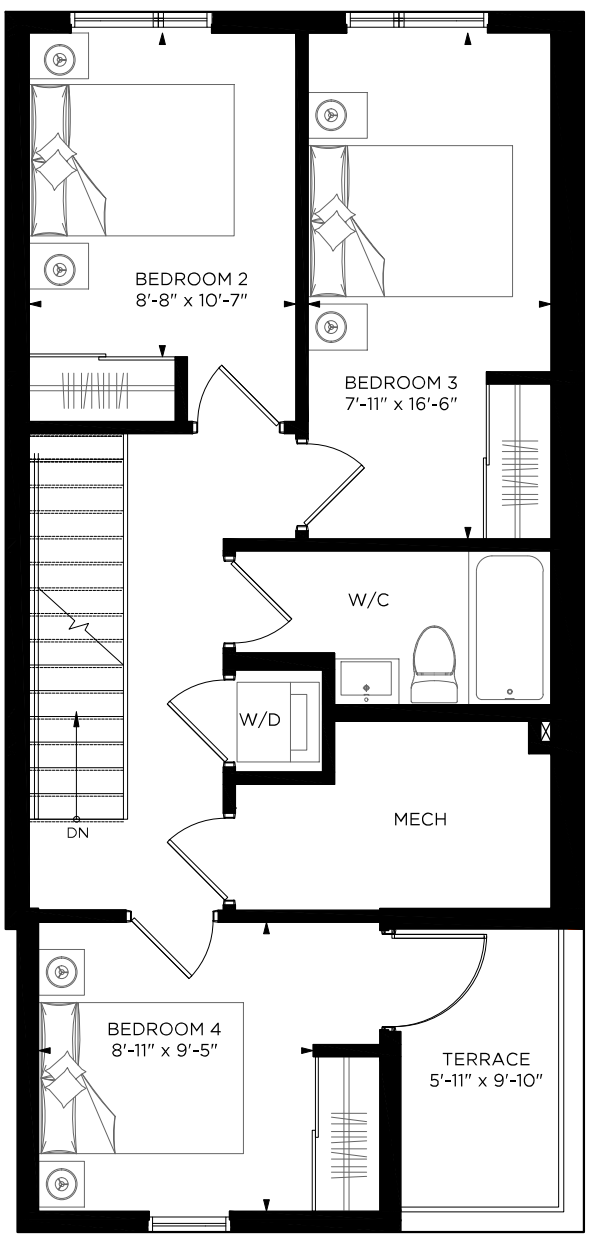
UPPER LEVEL THIRD FLOOR
